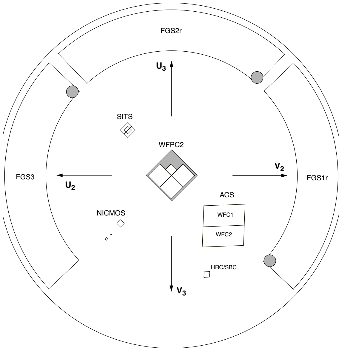
Figure 1.3: FGSs in the HST Focal Plane (Projected onto the Sky)
