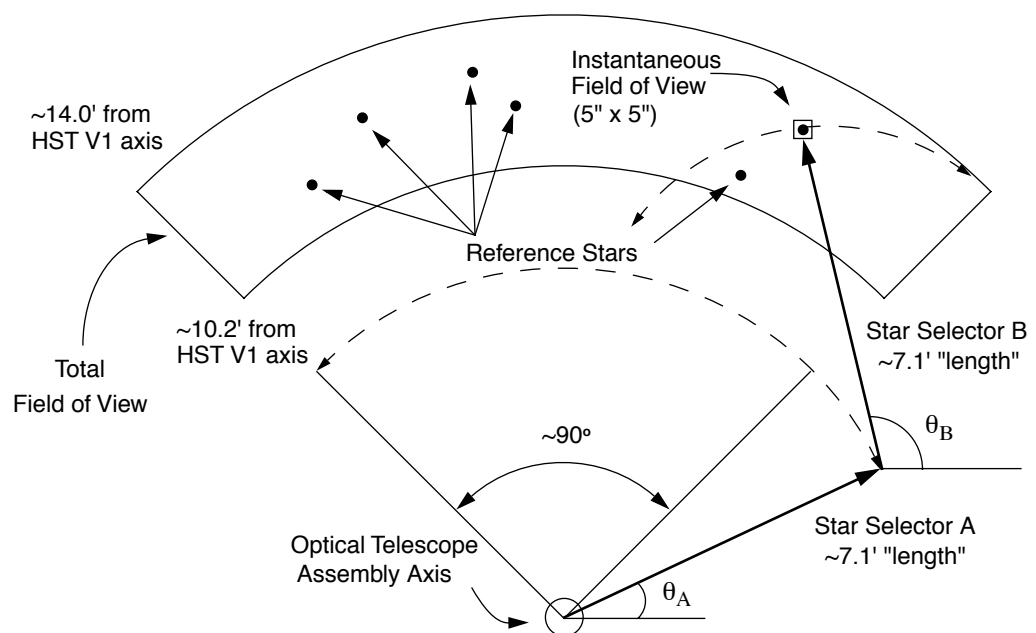
Figure 1.4: FGS Star Selector Geometry
