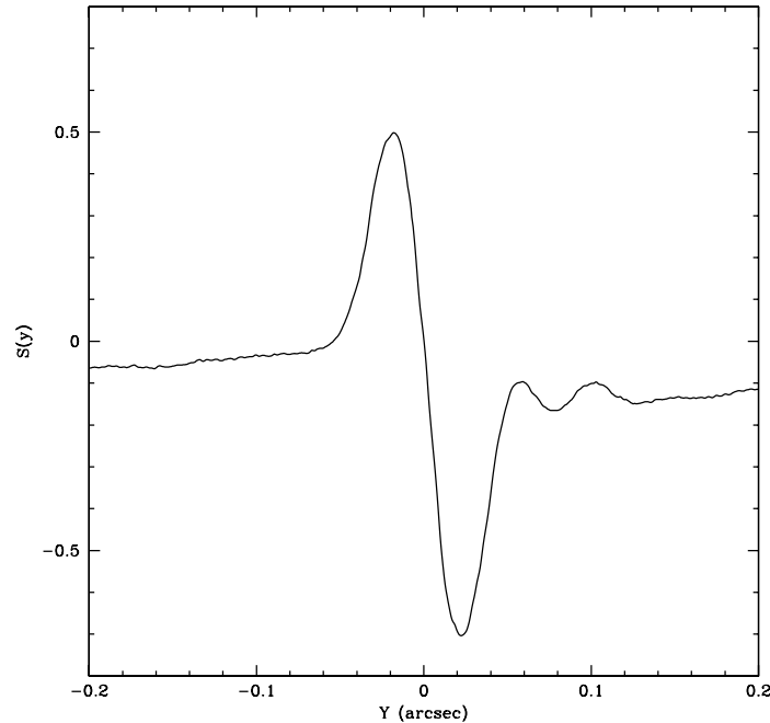
Figure 1.2: FGS Interferometric Response (the "S-Curve")
