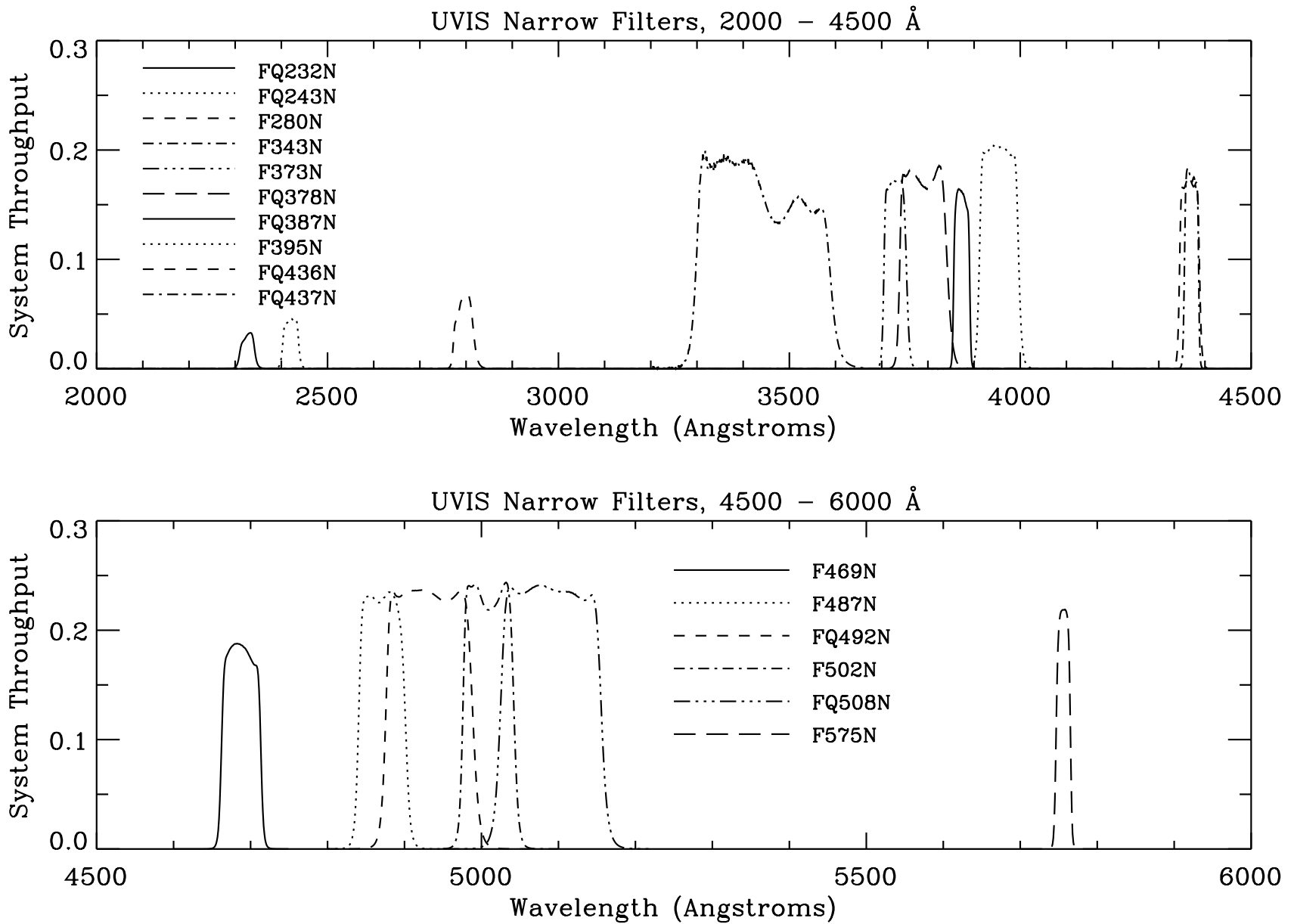
Figure 8: Integrated system throughput of the WFC3 UVIS narrow-band filters covering 2000-4500 Å (top panel) and the narrow-band filters covering 4500-6000 Å (bottom panel). The throughput calculations include the HST OTA, WFC3 UVIS-channel internal throughput, filter transmittance, and the QE of the UVIS flight detector.
