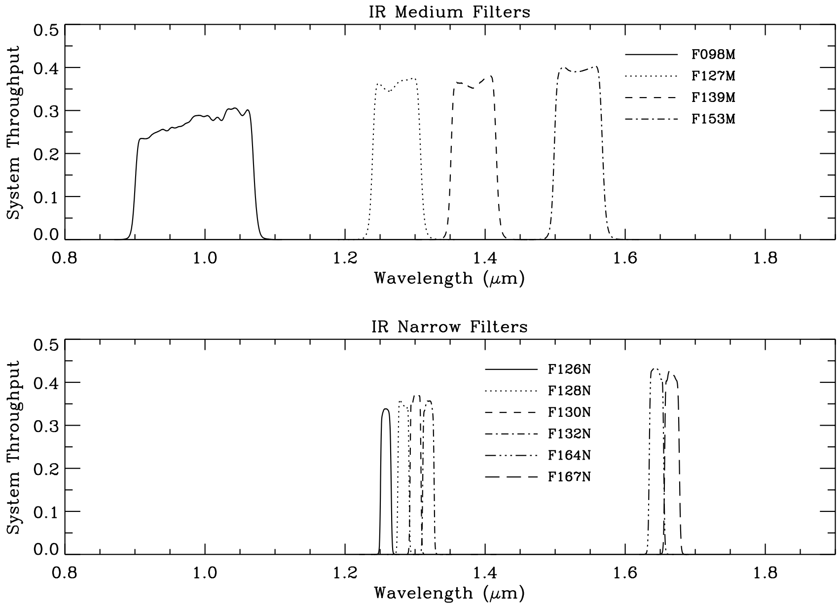
Figure 11: Integrated system throughput of the WFC3 IR medium-band filters (top panel) and narrow-band filters (bottom panel). The throughput calculations include the HST OTA, WFC3 IR-channel internal throughput, filter transmittance, and the QE of the FPA129 flight candidate IR detector.
