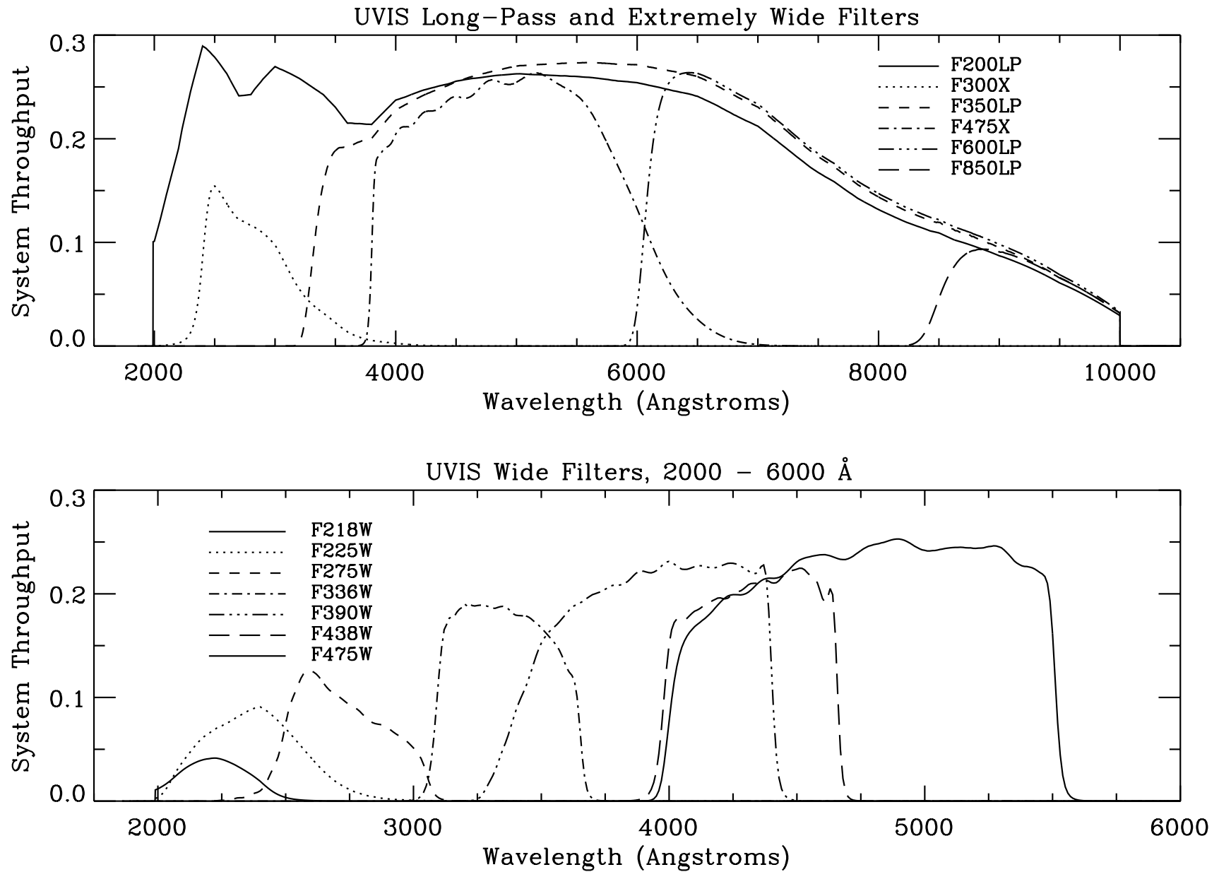
Figure 6: Integrated system throughput of the WFC3 UVIS long-pass and extremely wide filters (top panel) and of the wide-band filters covering 2000-6000 Å (bottom panel). The throughput calculations include the HST OTA, WFC3 UVIS-channel internal throughput, filter transmittance, and the QE of the UVIS flight detector. The short-wavelength cutoff at 2000 Å, and the long-wavelength cutoff at 10,000 Å, are artificial.
