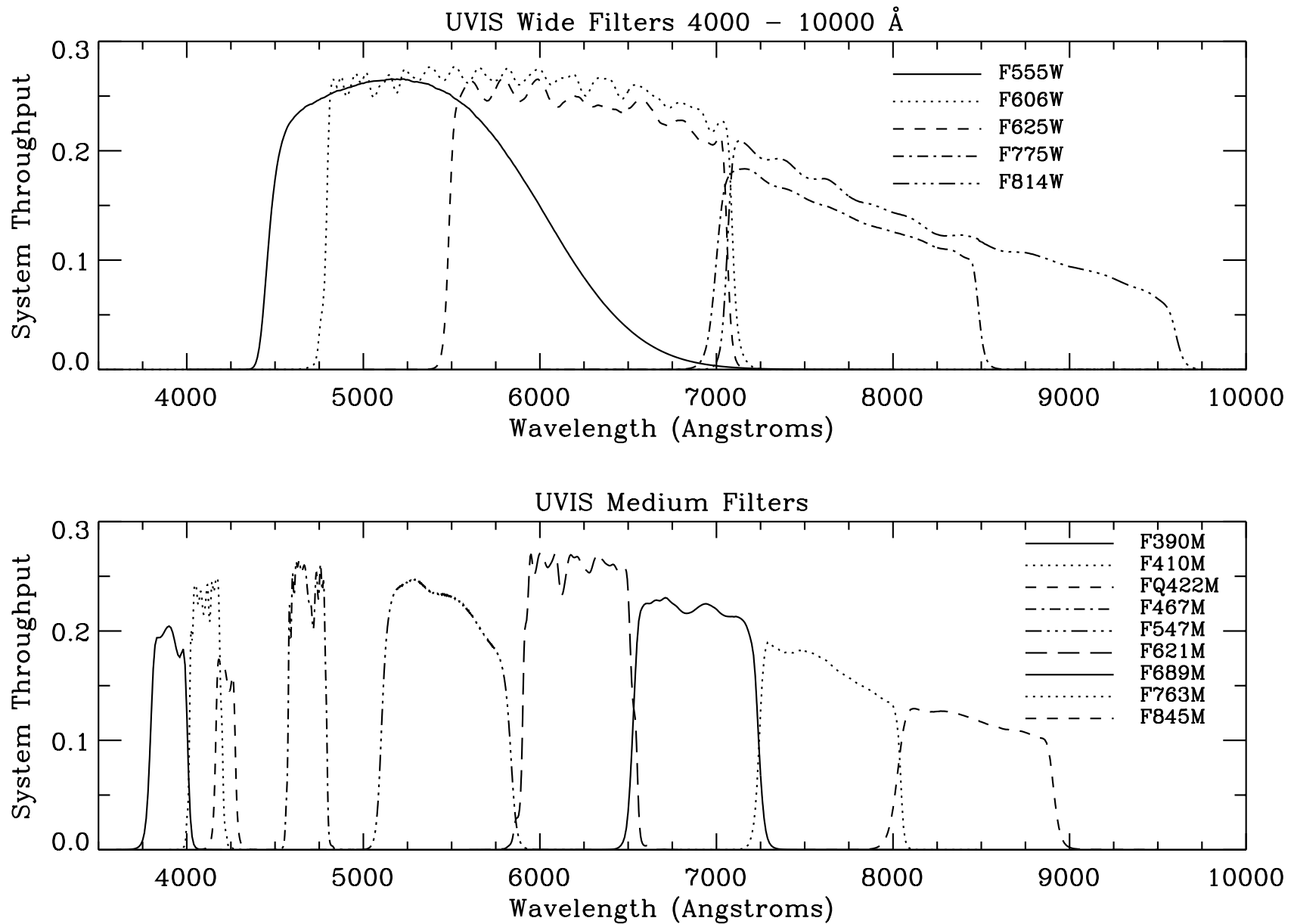
Figure 7: Integrated system throughput of the WFC3 UVIS wide-band filters covering 4000-10,000 Å (top panel) and the medium-band filters (bottom panel). The throughput calculations include the HST OTA, WFC3 UVIS-channel internal throughput, filter transmittance, and the QE of the UVIS flight detector.
