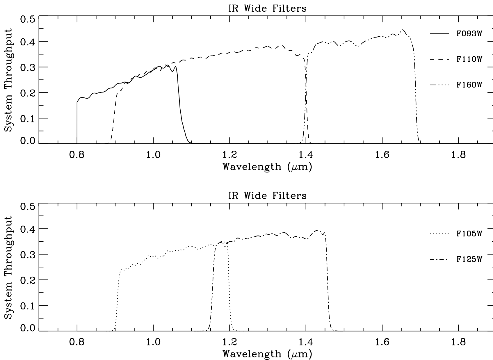
Figure 10: Integrated system throughput of the WFC3 IR wide-band filters, presented in two different panels for clarity. The throughput calculations include the HST OTA, WFC3 IR-channel internal throughput, filter transmittance, and the QE of the FPA129 flight candidate IR detector. The short-wavelength cutoff at 800 nm is artificial.
