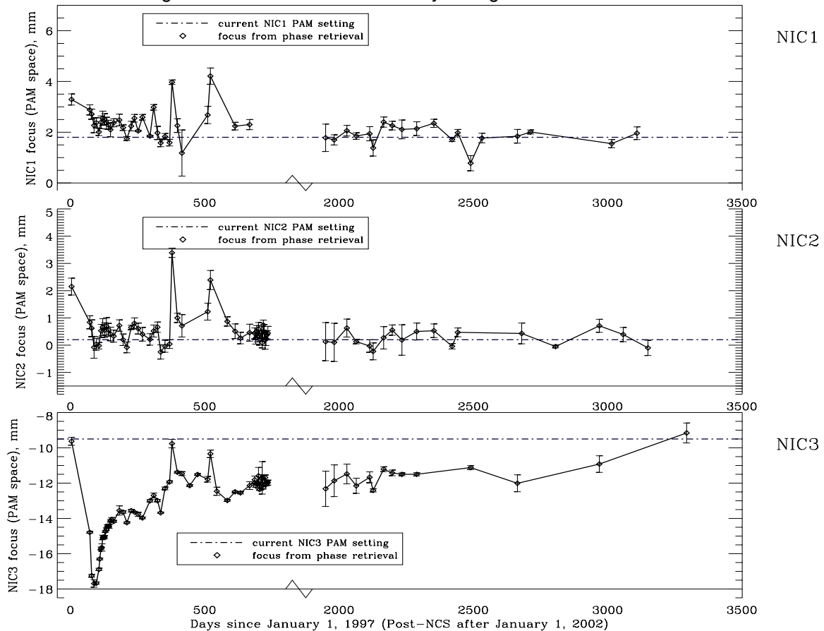
Figure 4.6: NICMOS Focus History through June 2006.
