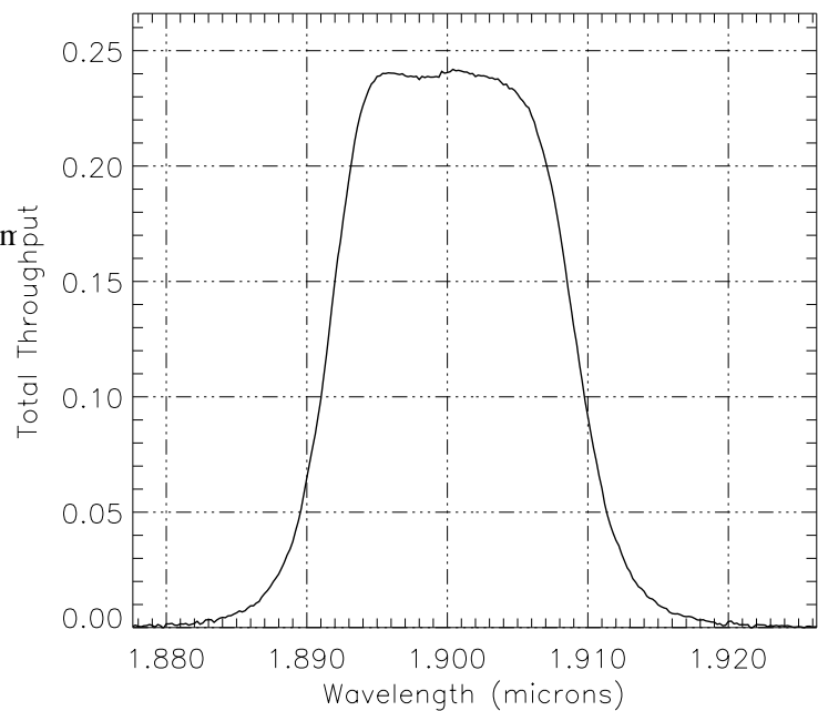
Figure A.44: NIC3, F190N Throughput
