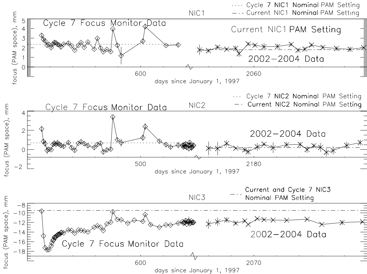
Figure 4.6: NICMOS Focus History through June 2004.
