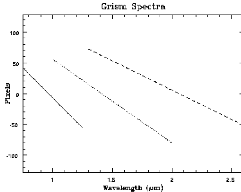
Figure 5.10: Wavelength Versus Pixel Number for each Grism. Note that the actual location of the central wavelength on the detector depends on the position of the source.
