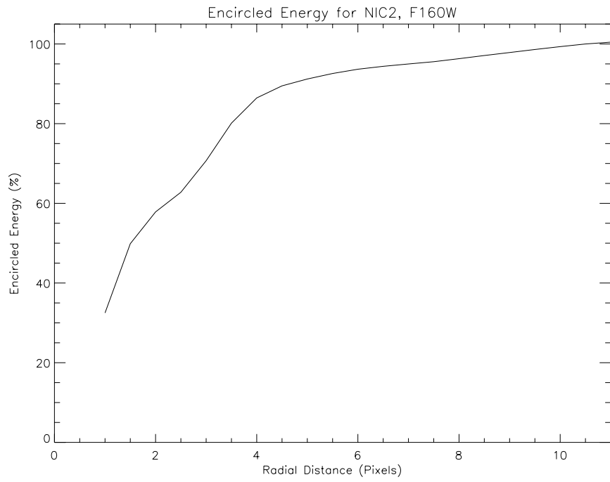
Figure 4.10: Encircled Energy for NIC2, F160W.
