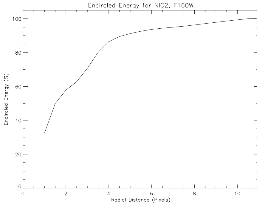
Figure 4.9: Encircled Energy for NIC2, F160W.
