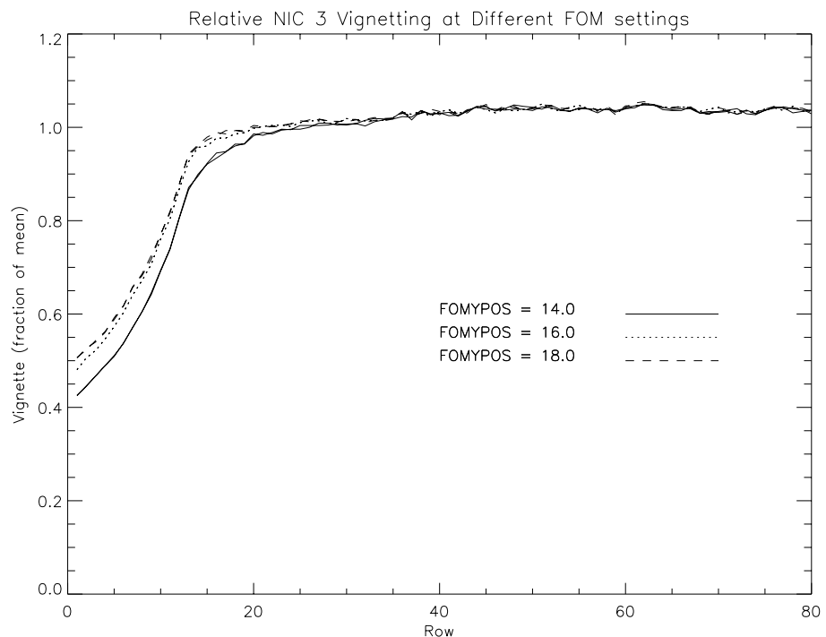
Figure 4.13: NIC3 Vignetting as a function of FOM offset.
