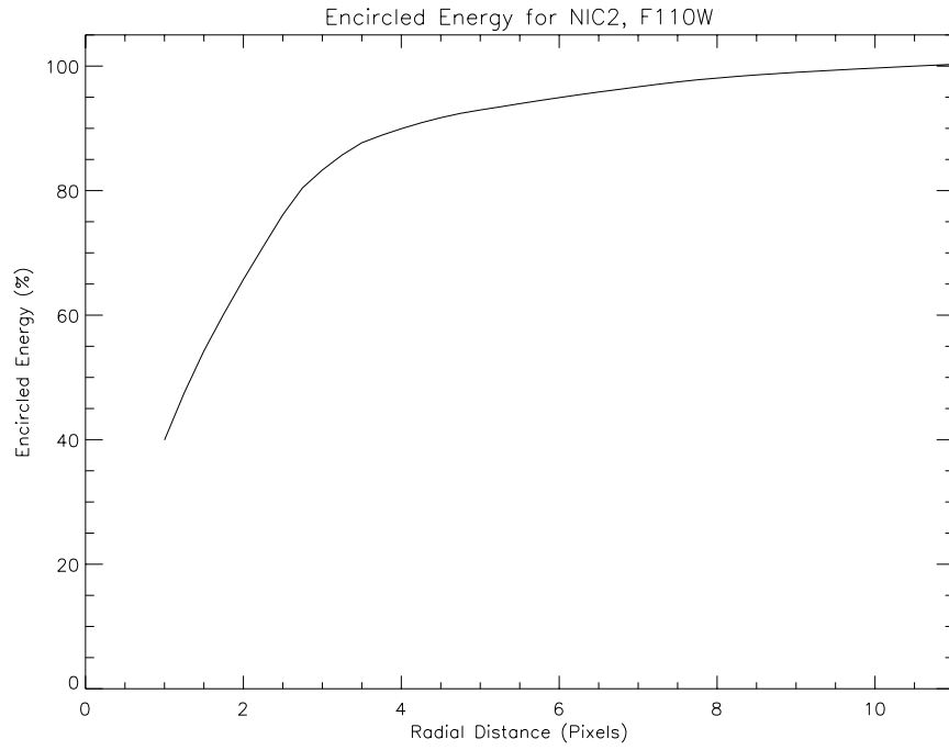
Figure 4.8: Encircled Energy for NIC2, F110W.
