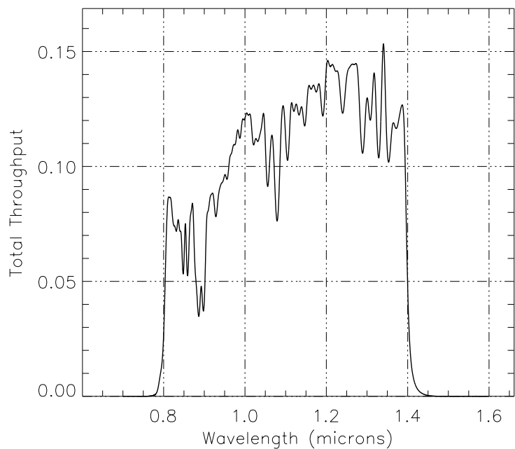
Figure A.36: NIC3, F110W Throughput
