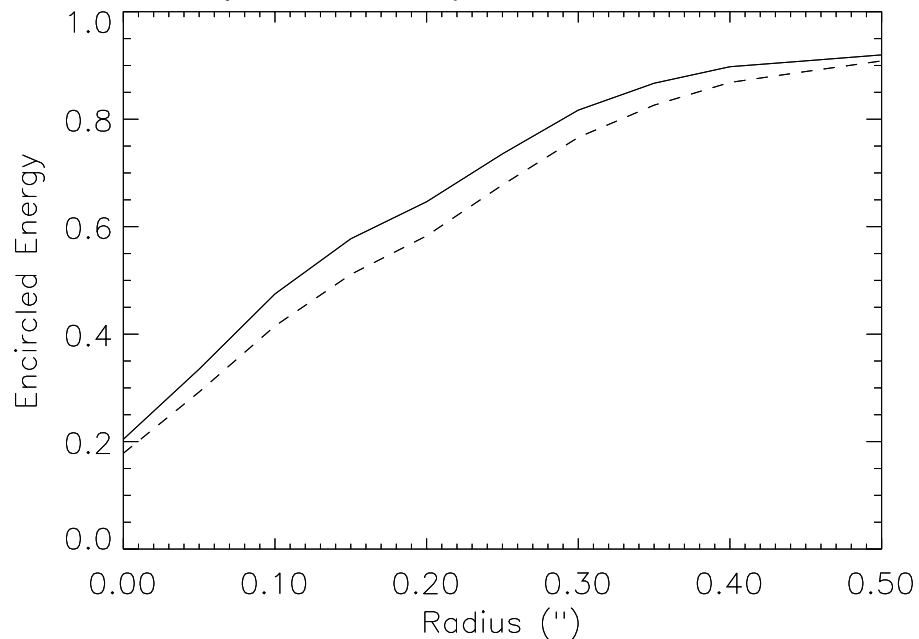
Figure 4.12: NIC3 encircled energy at 1.6 microns at optimum focus (PAM=-12 mm, solid line) and at the best achievable focus (PAM=-9.5 mm, dashed line) with the HST secondary mirror at nominal position.
