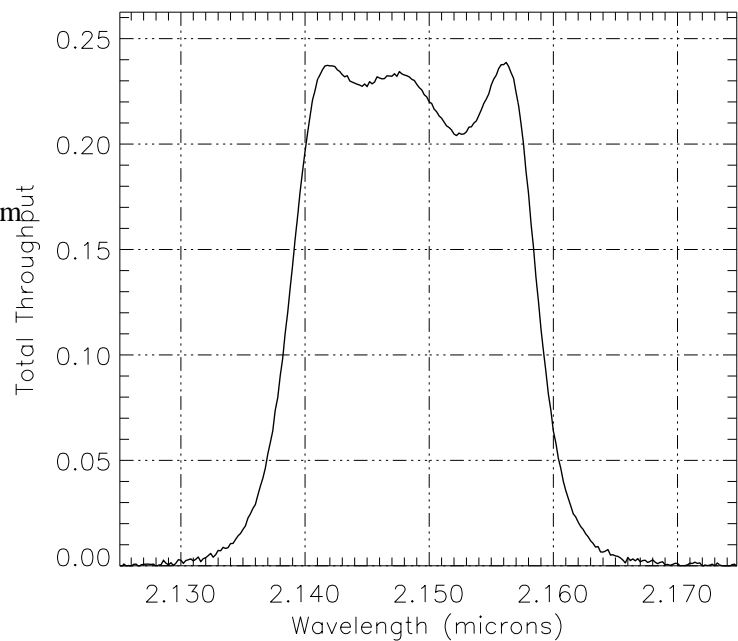
Figure A.48: NIC3, F215N Throughput
