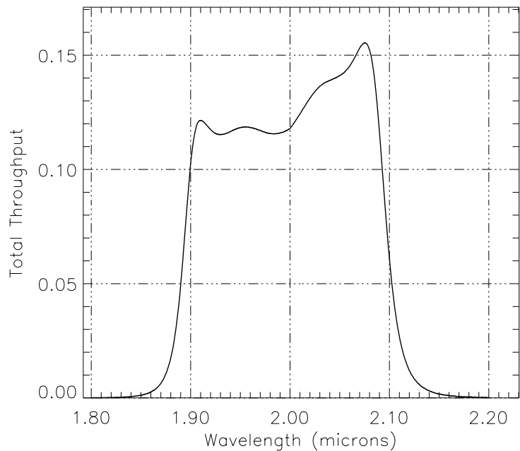
Figure A.34: NIC2, Long Polarizer Throughput
