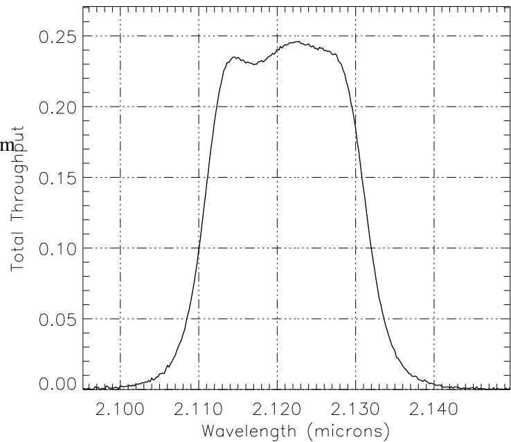
Figure A.47: NIC3, F212N Throughput
