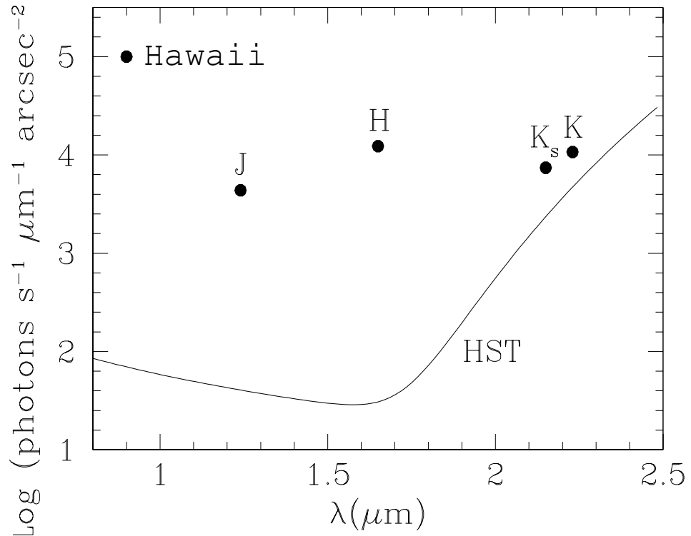
Figure 4.16: HST Background as seen by NICMOS. For comparison, the broad-band infrared background seen from Mauna Kea, Hawaii is shown.
