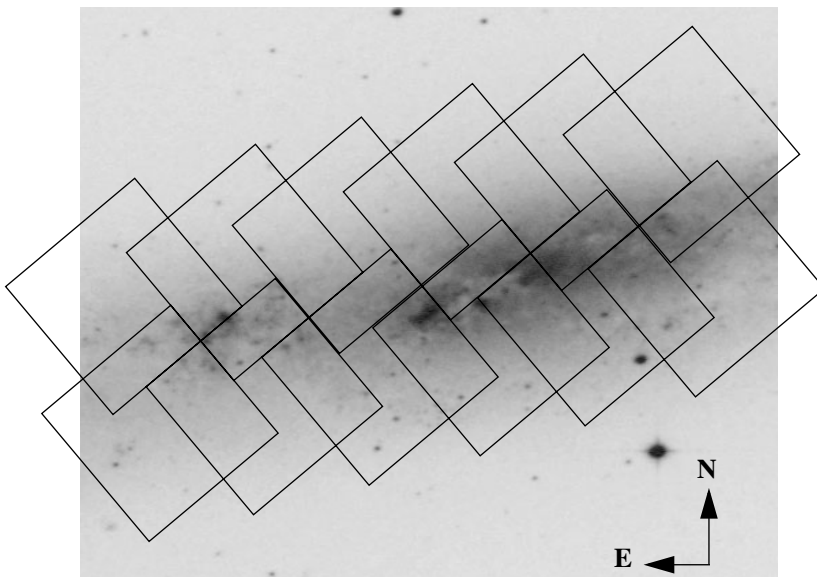
Figure 11.8: NIC-MAP Pattern
