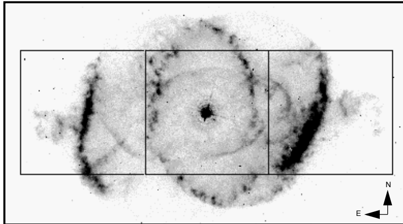
Figure 11.7: NIC-SKY-TWO-CHOP pattern.
