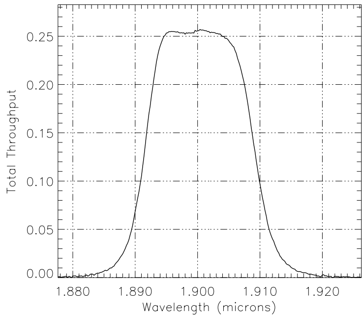
Figure A.25: NIC2, F190N Throughput
