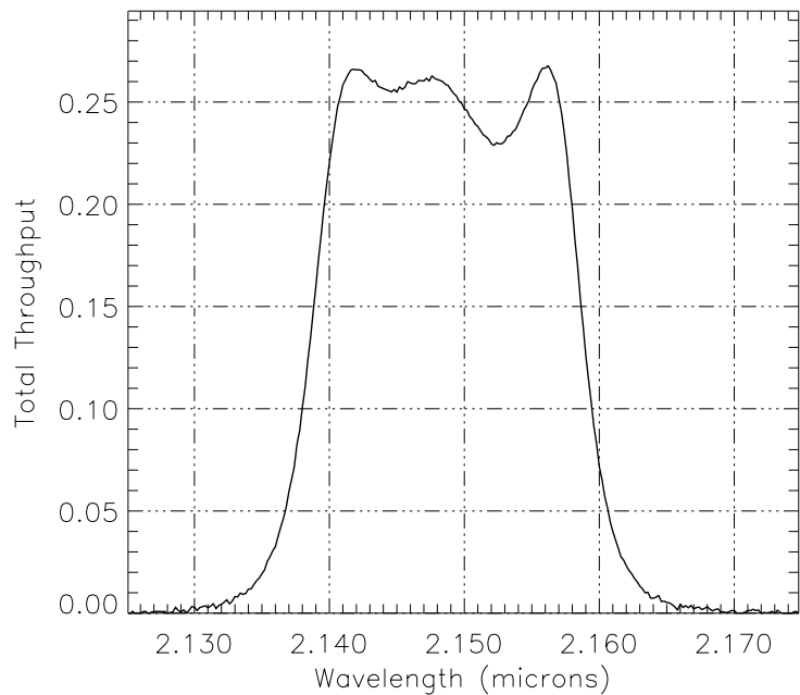
Figure A.30: NIC2, F215N Throughput
