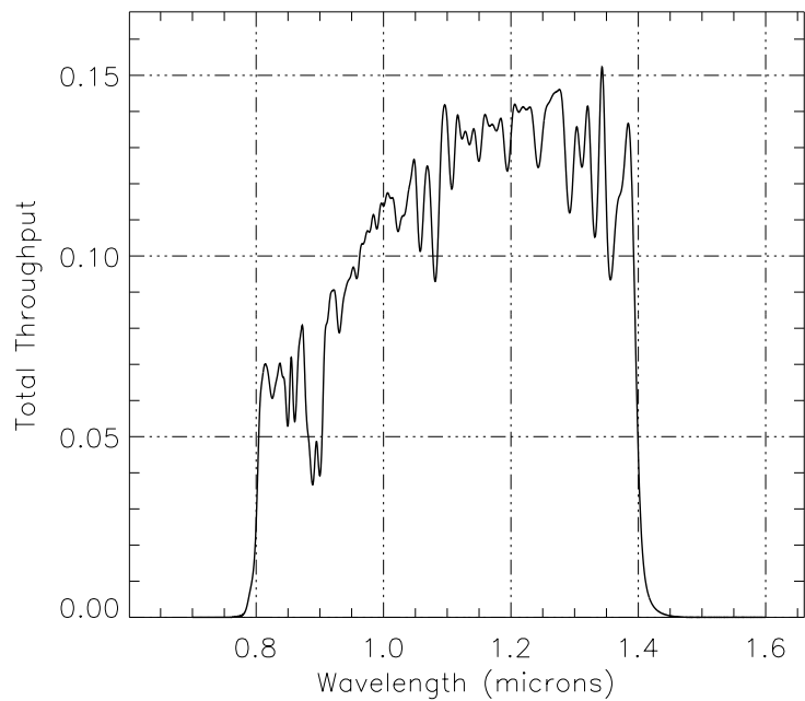
Figure A.6: NIC1, F110W Throughput
