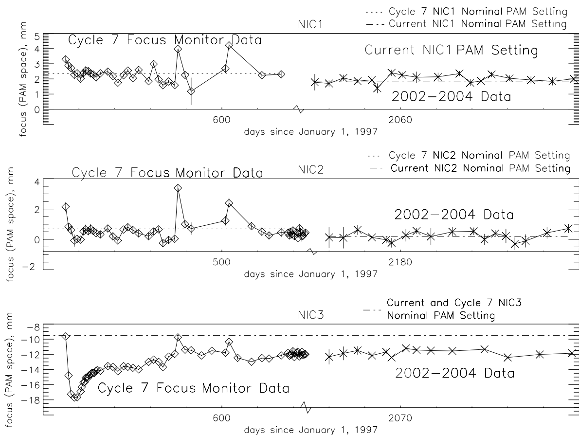
Figure 4.5: NICMOS Focus History through June 2004.
