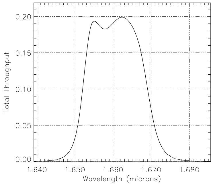
Figure A.13: NIC1, F166N Throughput
