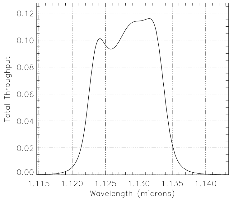
Figure A.37: NIC3, F113N Throughput
