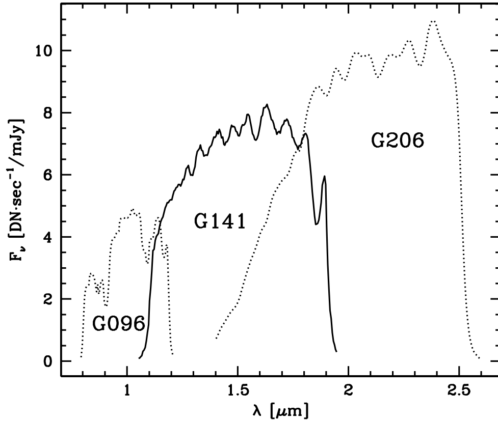
Figure 5.11: Grism Inverse Sensitivity Curves, G096 (left), G141 (middle), and G206 (right), measured with the post-NCS DQEs ( \sim 77.15\text{K} ).
