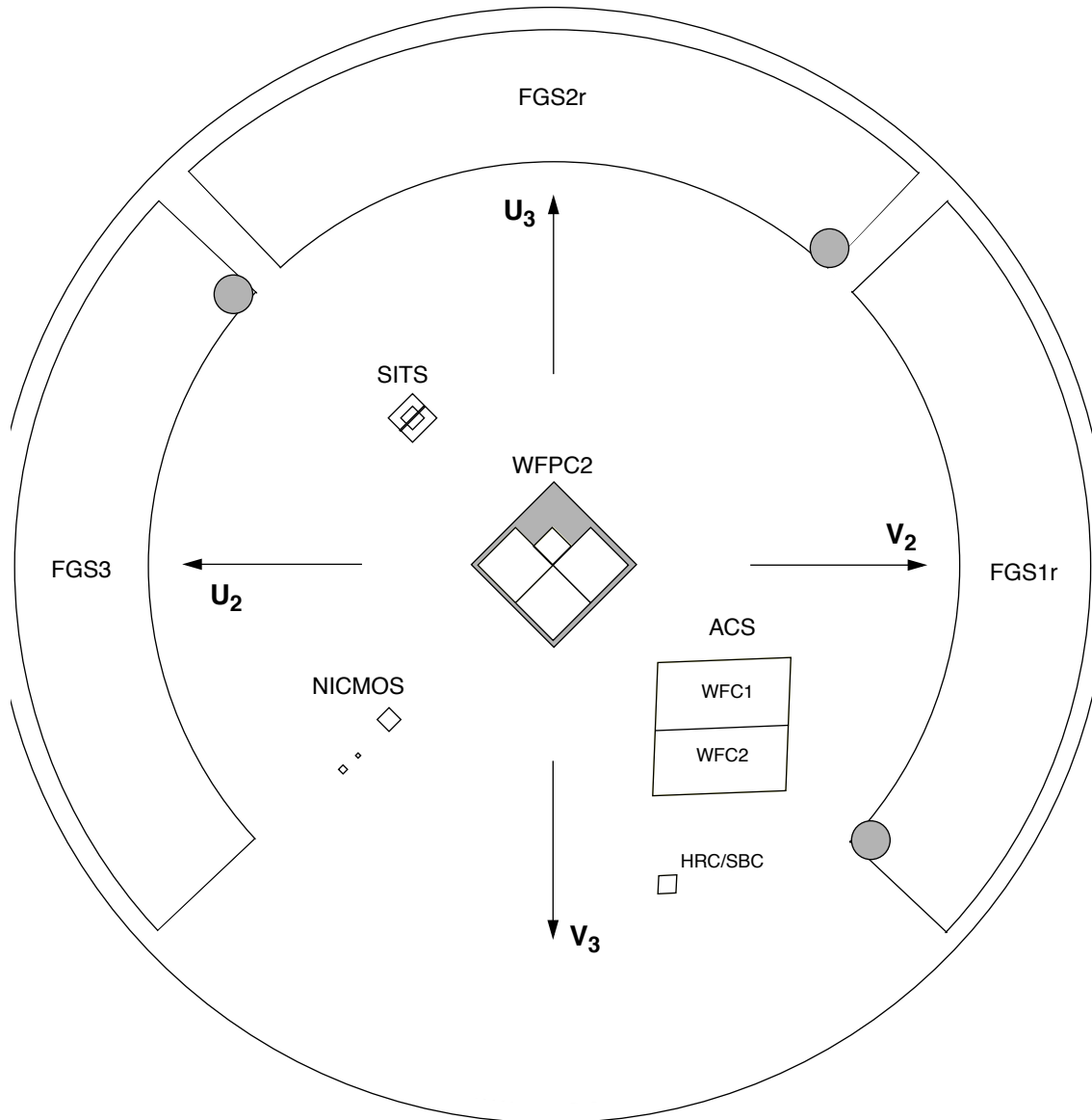
Figure 1.3: FGSs in the HST Focal Plane (Projected onto the Sky)
