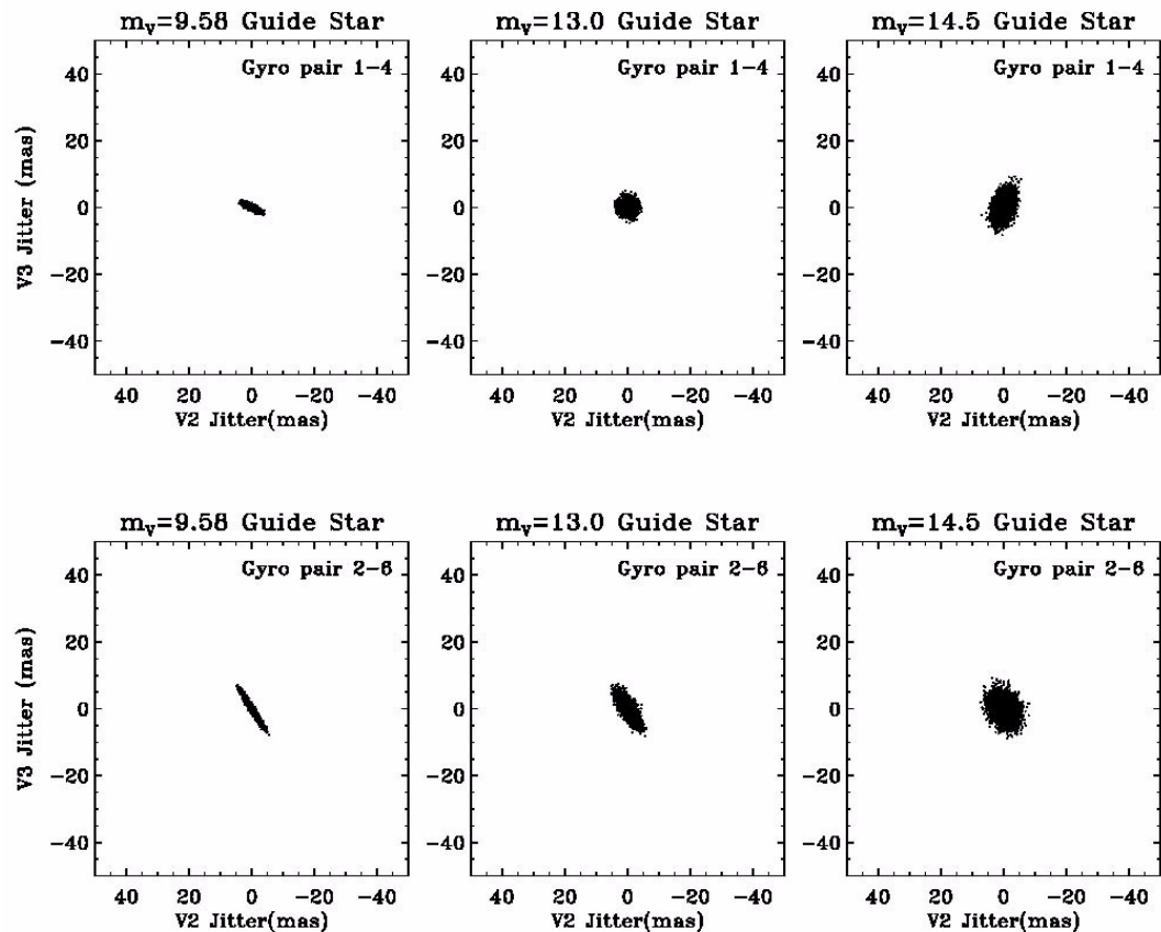
Figure 6.1: Jitter Ellipses Resulting from Rate Gyro Noise and FGS PMT Noise
