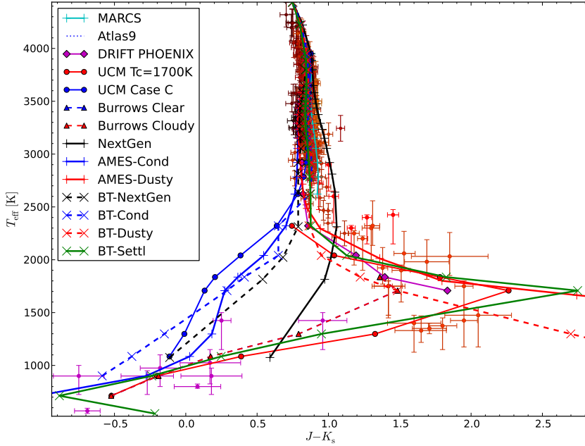
Fig. 4. Same as Fig. 2 but extending into the brown dwarf regime for an age of 3 Gyrs. The region below 2900 K is dominated by dust formation. The dust free models occupy the blue part of the diagram and only at best explain T dwarf colors, while the Dusty and DRIFT models explain at best L dwarfs, becoming only redder with decreasing T_{\text{eff}} . The BT-Settl, Cloudy and UCM T_{\text{crit}} = 1700 K models describe a complete transition to the red in the L dwarf regime before turning to the blue into the T dwarf regime, only the BT-Settl extends into the Y dwarfs regime ( T_{\text{eff}} \leq 500 K).
