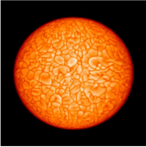
Fig. 3. Global RHD simulation of an M dwarfs with solar composition. Obtained parameters are T_{\text{eff}} = 3143.44 K, \log g = 4.38 , and a radius of 0.003 R_{\odot} . The surface pressure is 68227.6 \text{ g/cm}^2 , the surface density is 4.52146e-07 \text{ g/cm}^3 , the central temperature is 28889.7 K, the central pressure is 1.67214e+09 \text{ g/cm}^2 , the central density is 6.92703e-4 \text{ g/cm}^3 . The model covers 10 pressure scale heights from the center to the surface. The simulations use grey PHOENIX opacities in the outer layers merged with OPAL data for the interior layers. The rotation period of the simulation is 1 hour and the simulation is shown equator-on in the reference frame of rotation. One can notice a slight oblateness of the model at this exaggerated velocity for an M dwarf.
