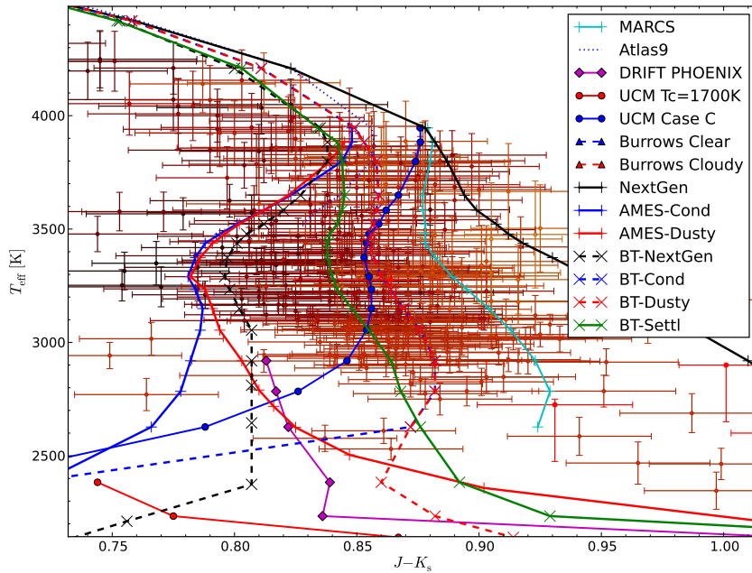
Fig. 2. Estimated T_{\text{eff}} and metallicity (decreasing from lighter to darker tones) for M dwarfs by Casagrande et al. (2008a) on the left, and brown dwarfs by Golimowski et al. (2004) and Vrba et al. (2004) on the right are compared to the NextGen isochrones for 5 Gyrs Baraffe et al. (1998) using model atmospheres by various authors: MARCS by Gustafsson et al. (2008), ATLAS9 by Castelli & Kurucz (2004), DRIFT-PHOENIX by Helling et al. (2008), UCM by Tsuji (2002), Clear/Cloudy by Burrows et al. (2006), NextGen by Hauschildt et al. (1999), AMES-Cond/Dusty by Allard et al. (2001), the BT-Cond/Dusty/NextGen models by Allard et al. (2012) and the current BT-Settl models. Some curves labeled in the legend can only be seen in the more extended Fig. 4.
